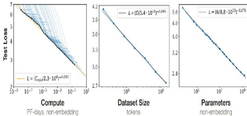
Figure 1 Language modeling performance improves smoothly as we increase the model size, dataset size, and amount of compute 2 used for training. For optimal performance all three factors must be scaled up in tandem. Empirical performance has a power-law relationship with each individual factor when not bottlenecked by the other two.
